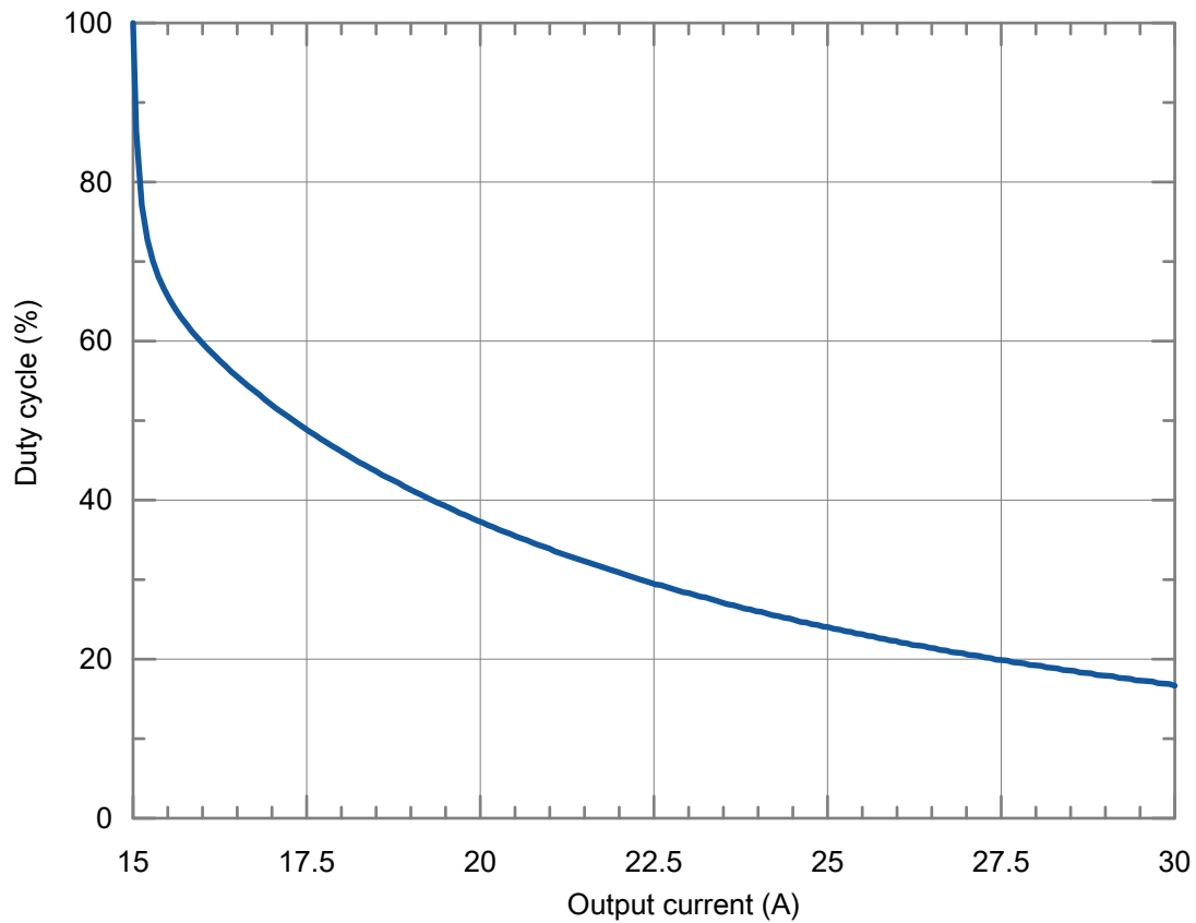
Figure 1-6: Output duty cycle limit over current amplitude
