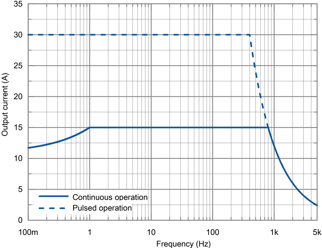
Figure 1-7: Current output derating over frequency
