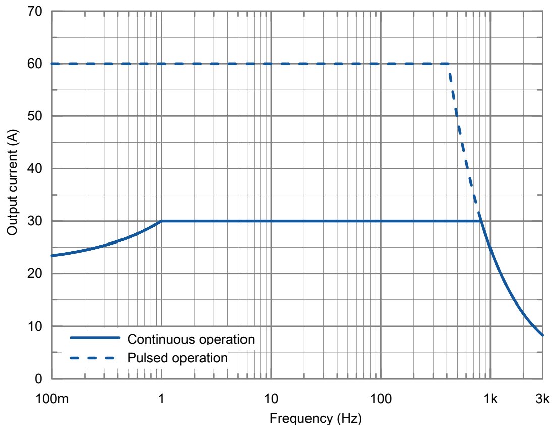
Figure 1-13: Current output derating over frequency
