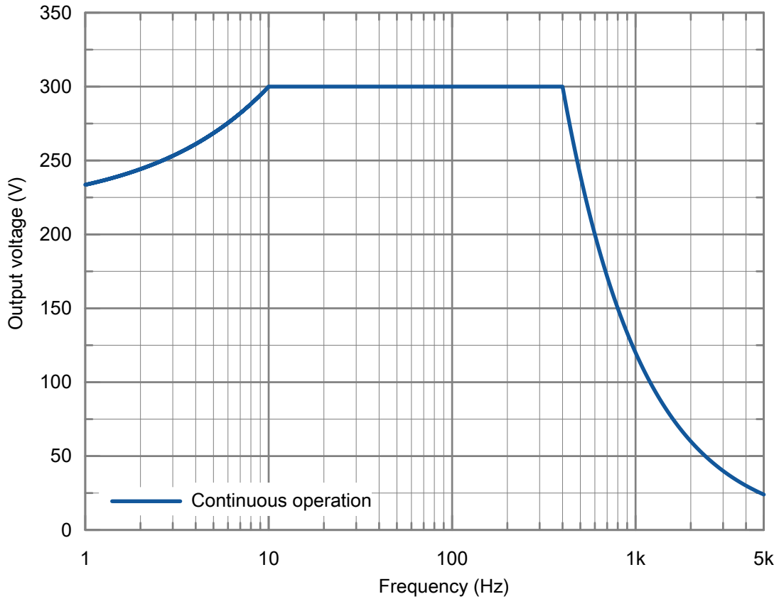
Figure 1-8: Voltage output derating over frequency
