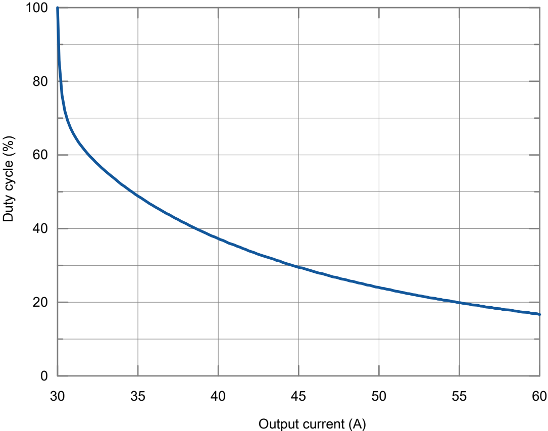
Figure 1-12: Output duty cycle limit over current amplitude
