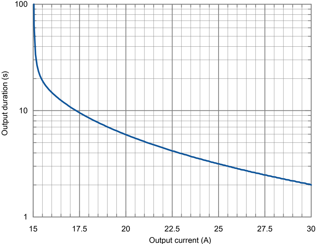
Figure 1-5: Output duration limit over current amplitude
